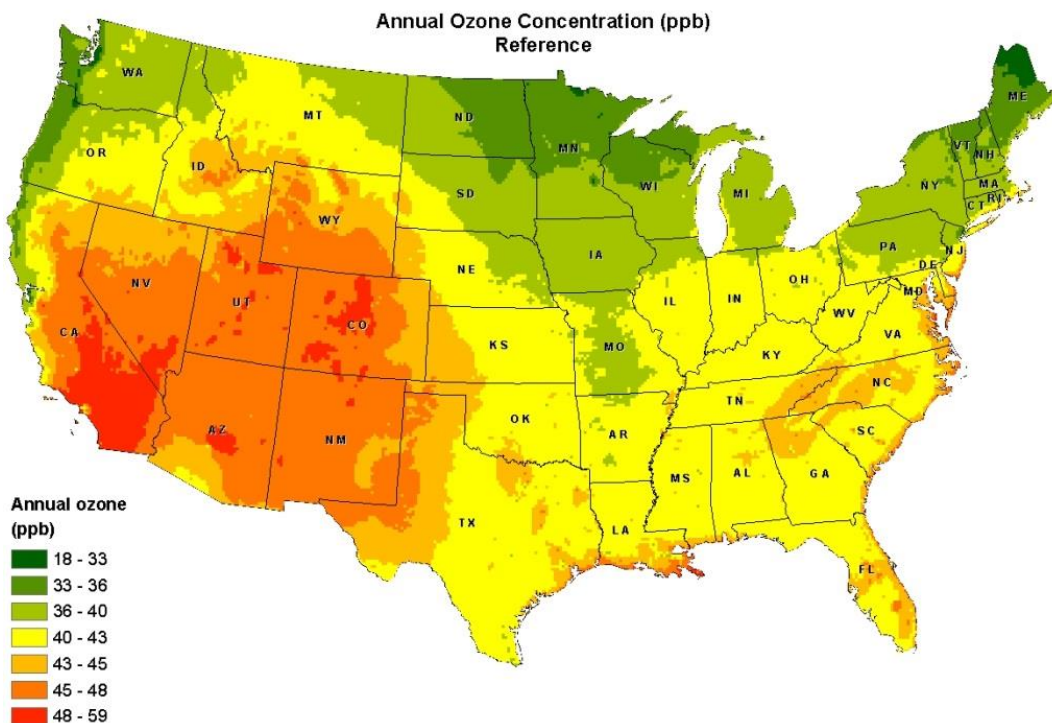
Figure 9a & b: Average annual peak 8-hr ozone for Reference Case and change in this condition for Scenario #2 (parts per billion).
